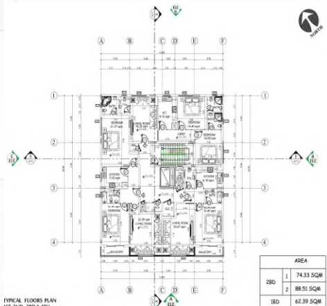
TYPICAL FLOORS PLAN 1ST, 2ND, 3RD & 4TH
